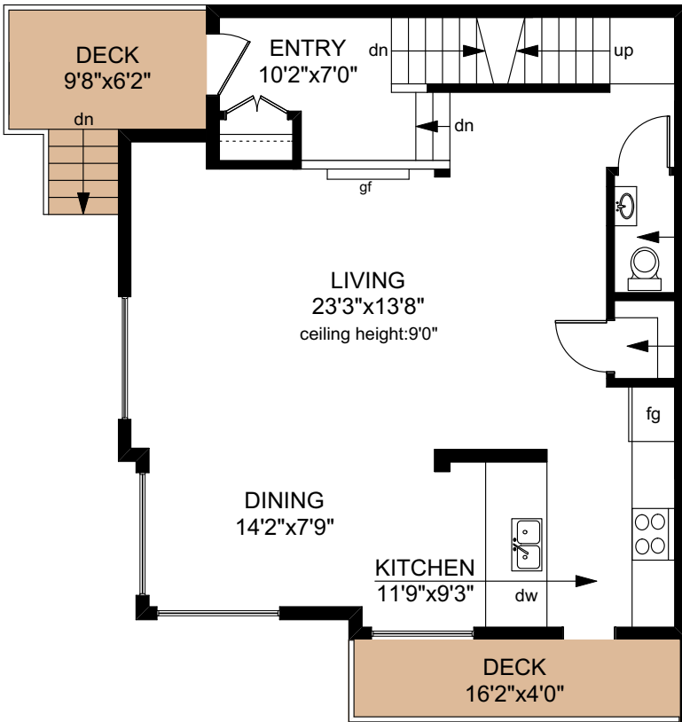
MAIN FLOOR 752 SQ.FT
