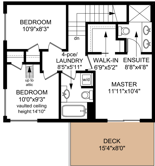
UPPER FLOOR 545 SQ.FT
